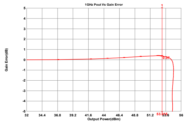
1GHz Gain Error Curve, passes +/-1dB
